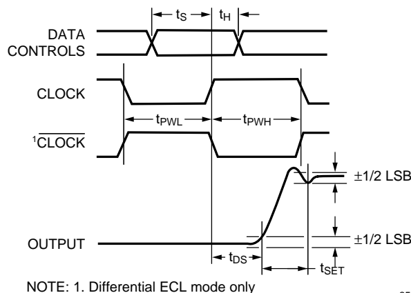
Figure 1. Timing Diagram
